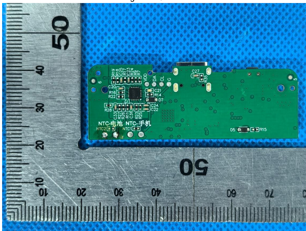
Fig. 8 – PCB view
