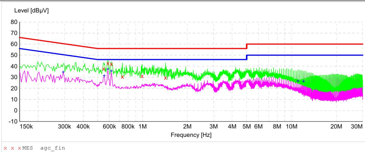
Test graph and data for Conducted Emission Test Mode: Mode 3
