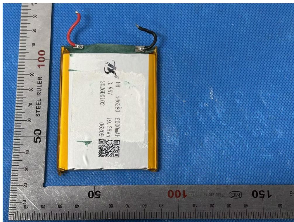
Fig. 7 – Battery view
