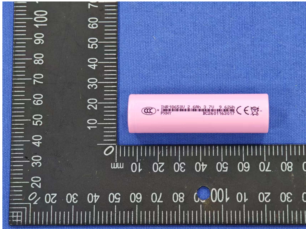
Picture 1 Front view of cell (Model: INR18650V)
