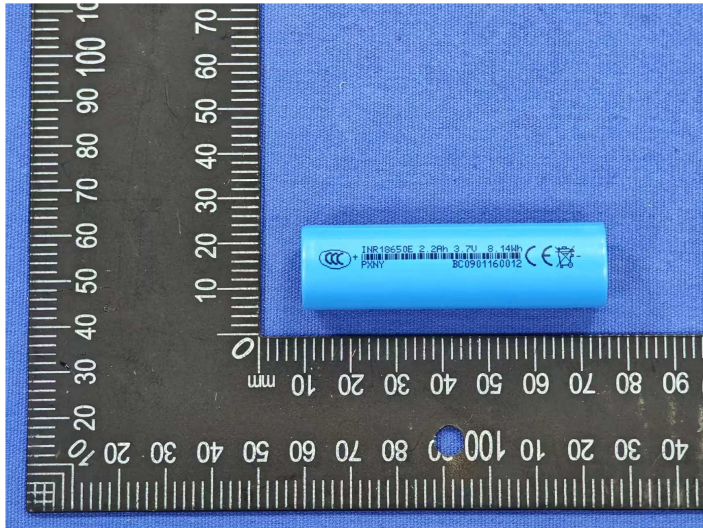
Picture 9 Front view of cell (Model: INR18650E)
