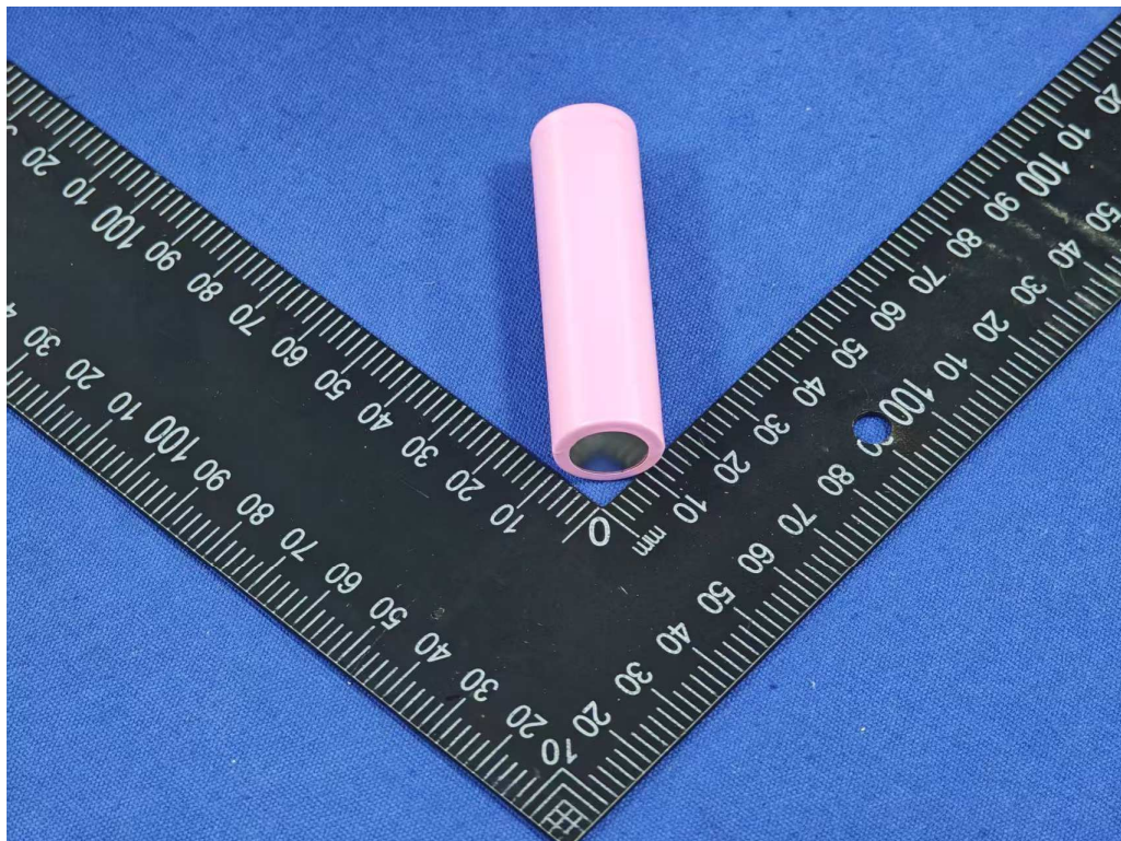
Picture 4 Bottom view of cell (Model: INR18650V)
