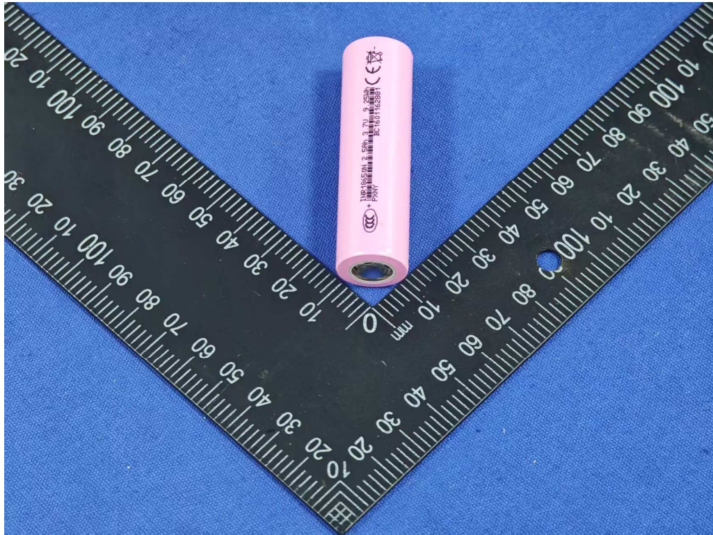
Picture 7 Top view of cell (Model: INR18650N)
