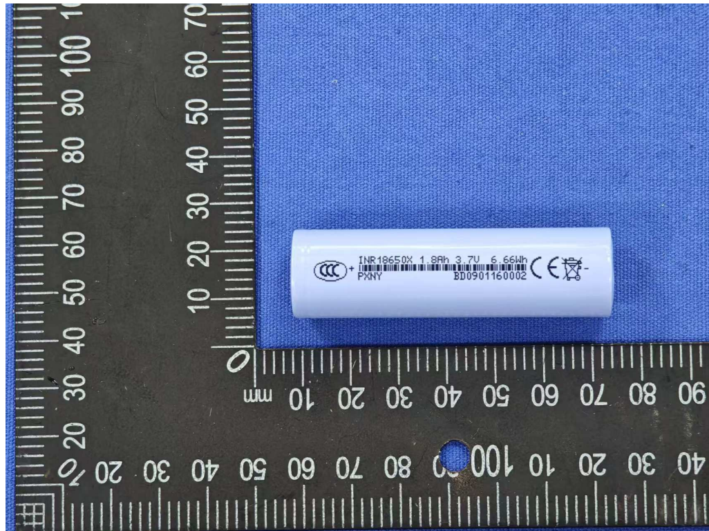
Picture 13 Front view of cell (Model: INR18650X)
