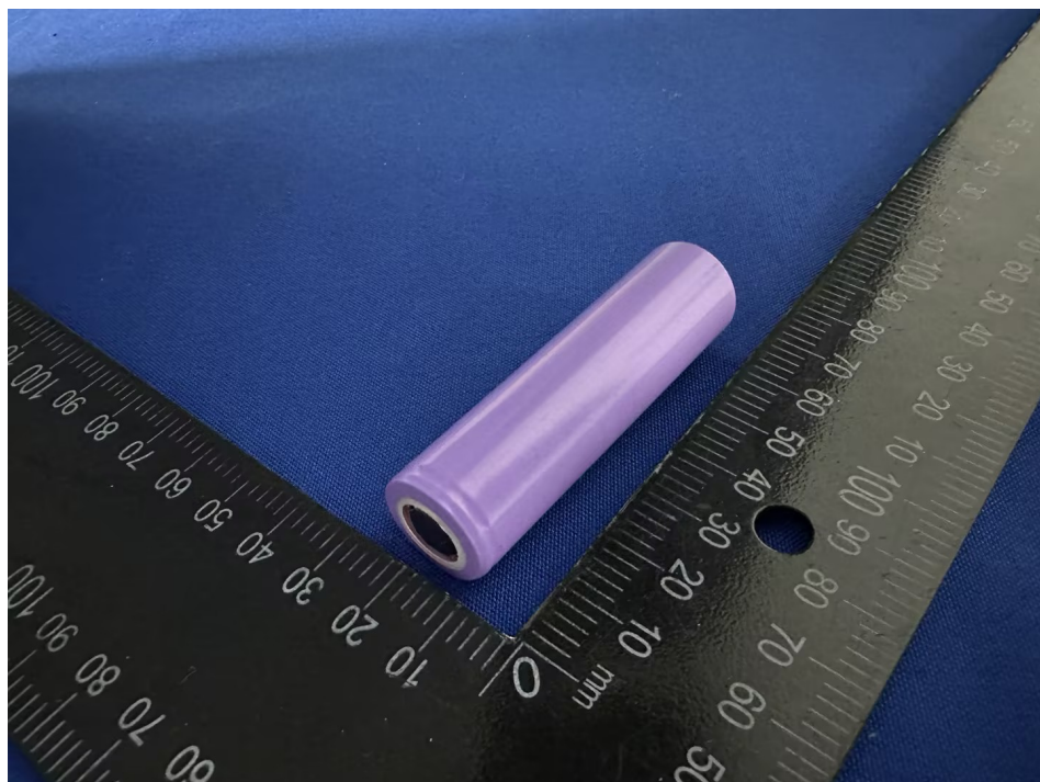
Picture 6. Side view-2 of cell for model HYLN IMR18650-2000mAh
