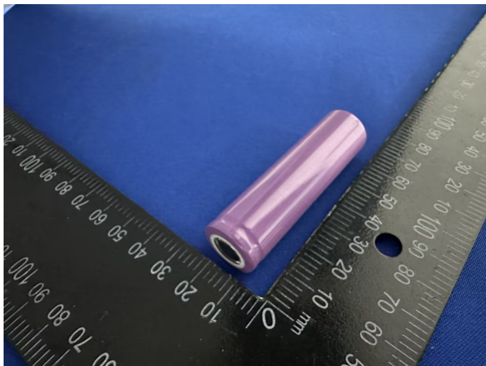
Picture 14. Side view-2 of cell for model HYLN IMR18650-1200mAh
