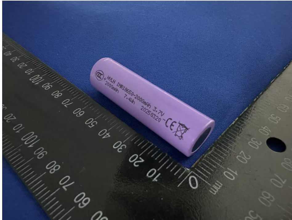
Picture 5. Side view-1 of cell for model HYLN IMR18650-2000mAh
