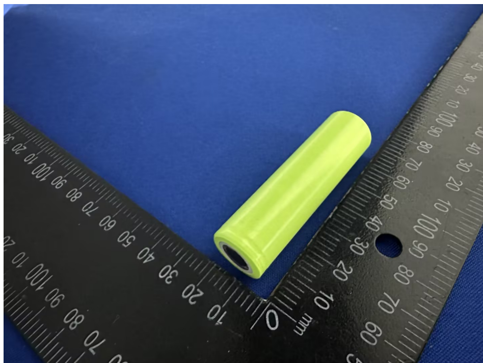
Picture 4. Side view-2 of cell for model HYLN IMR18650-2500mAh
