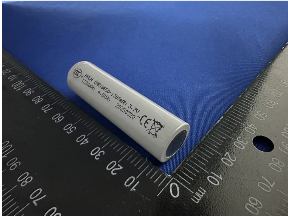
Picture 11. Side view-1 of cell for model HYLN IMR18650-1300mAh
