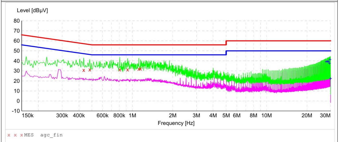
Test graph and data for Conducted Emission Test Mode: Mode 2
