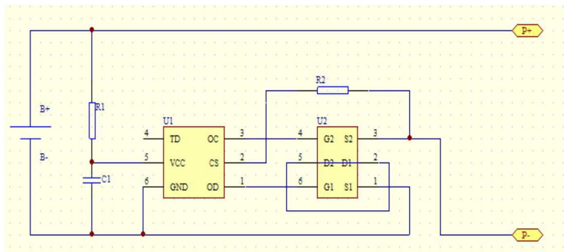
Circuit diagram
