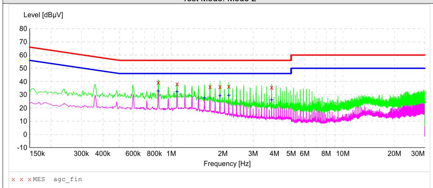
Test graph and data for Conducted Emission
