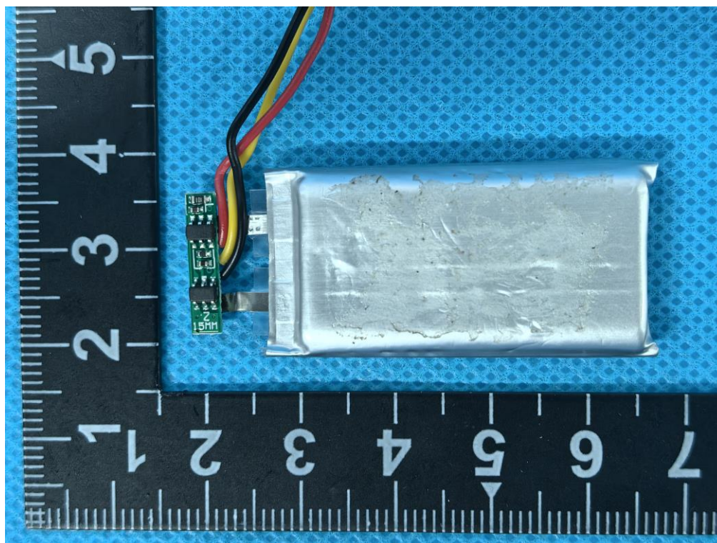
Fig. 11 – Battery view
