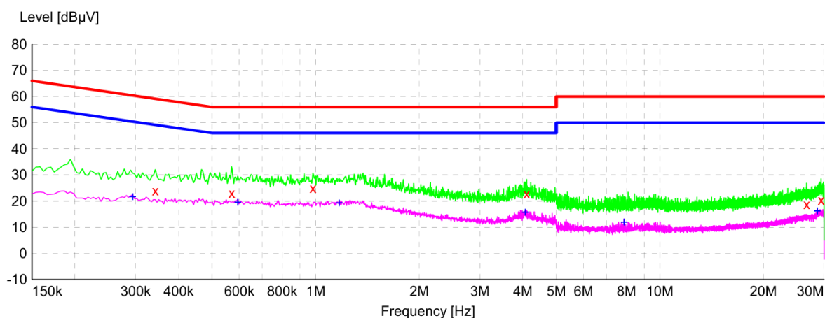
Test graph and data for Conducted Emission
