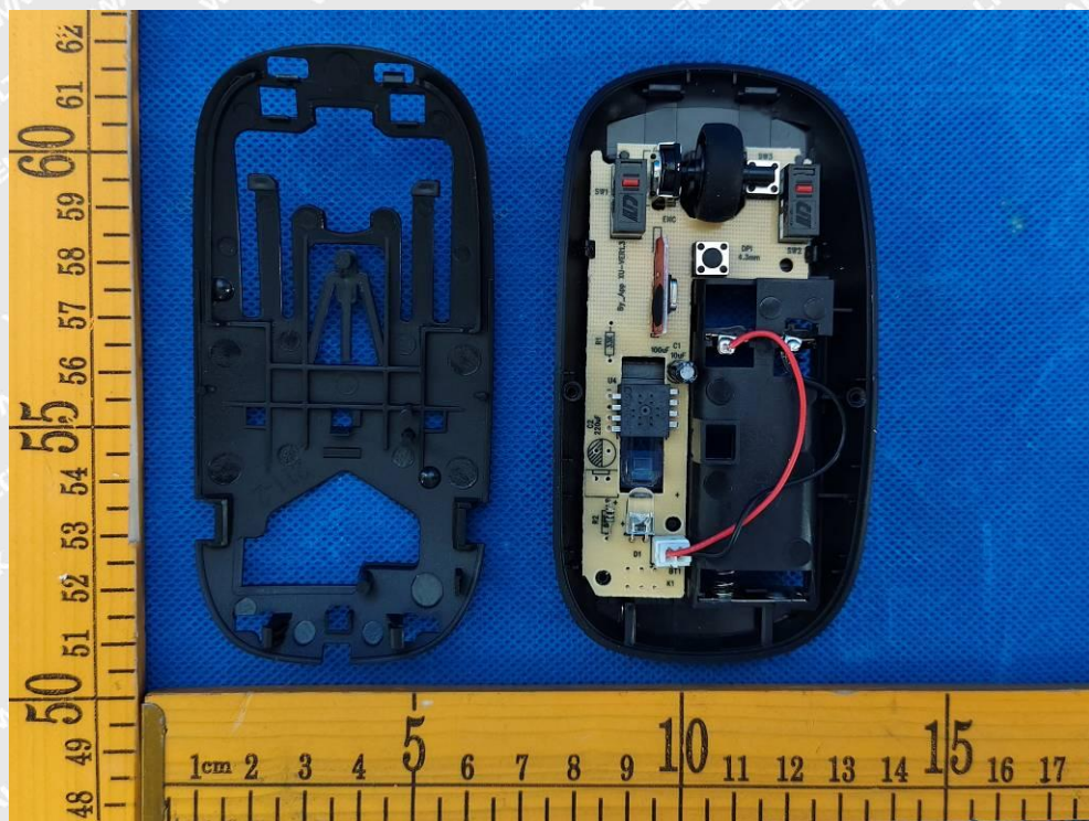
Photo 5: Internal view
