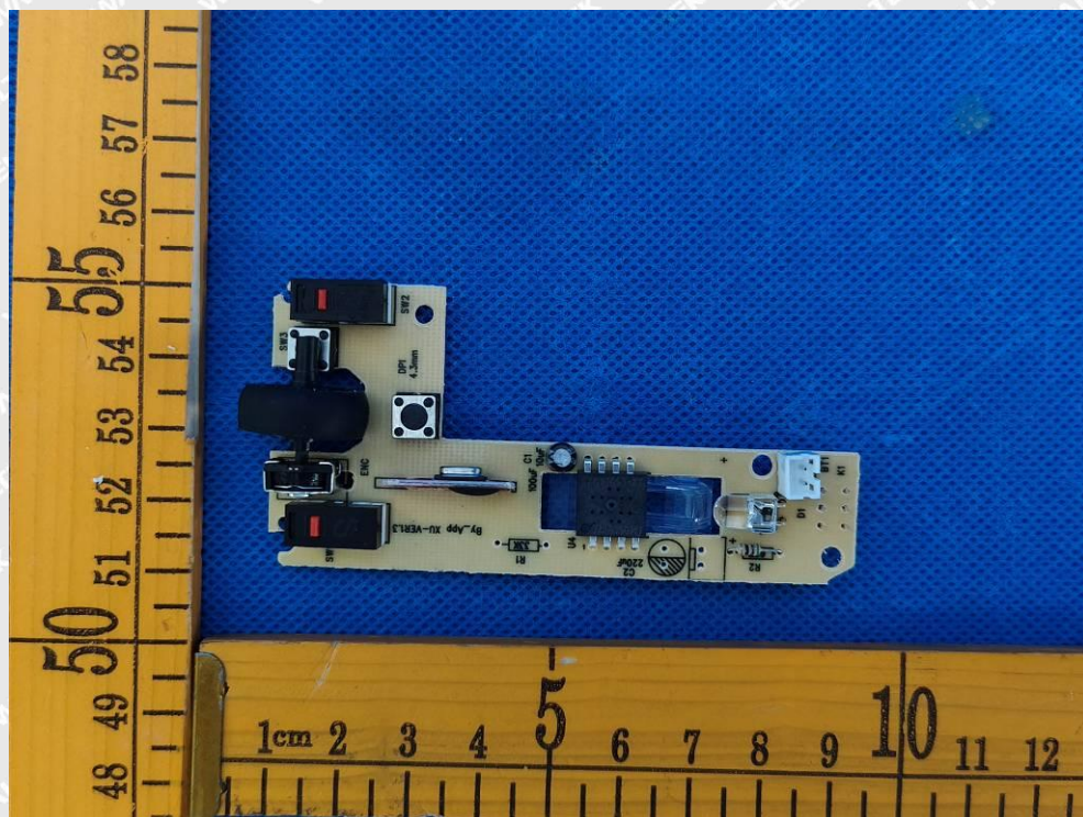
Photo 7: PCB view
