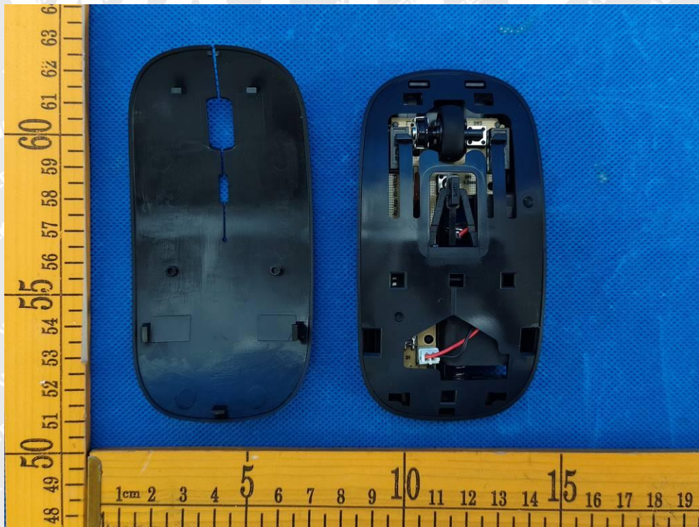
Photo 3: Internal view
