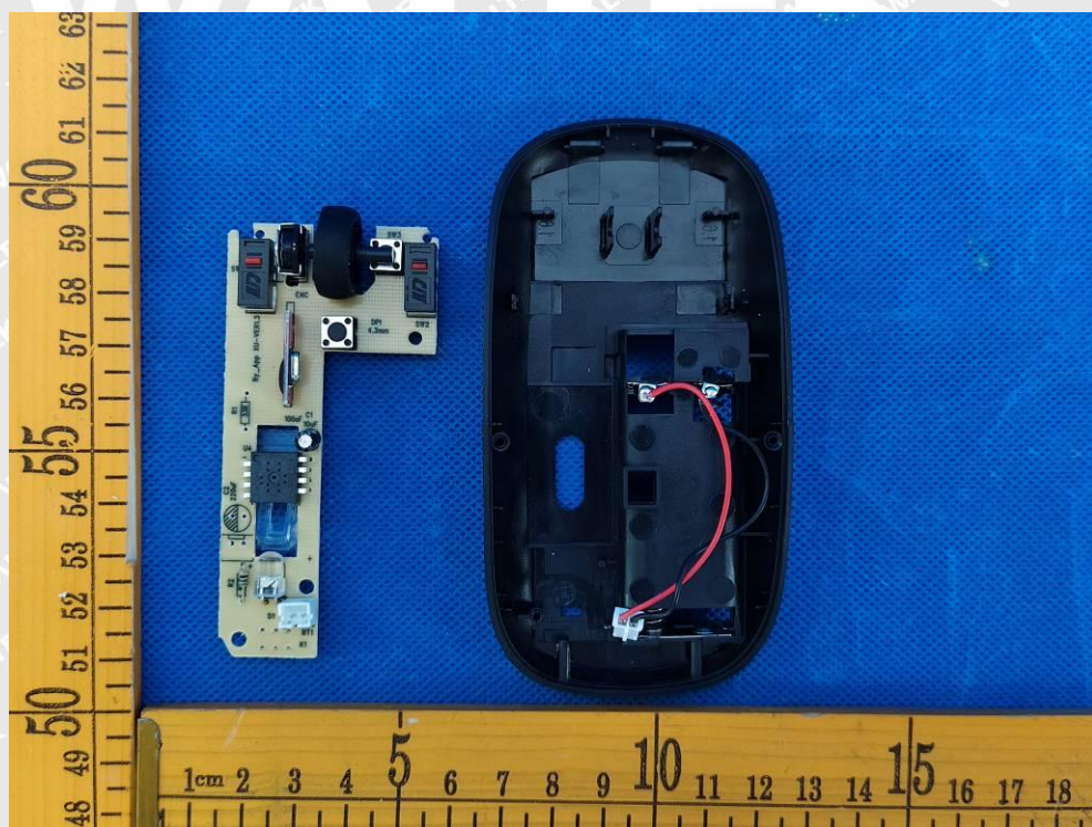
Photo 6: Internal view
