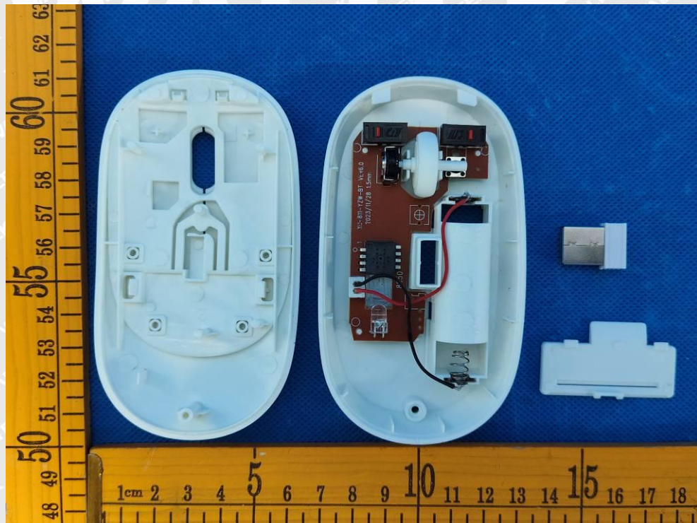
Photo 3: Internal view
