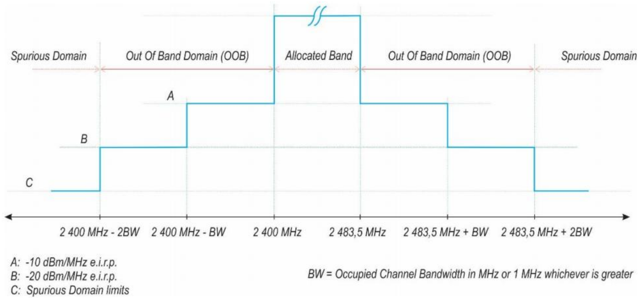
Figure 1: Transmit mask
