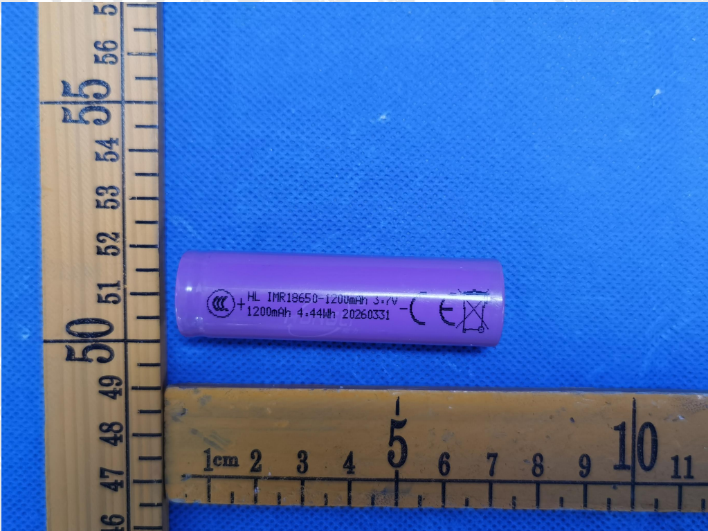
Figure 8 Battery view
