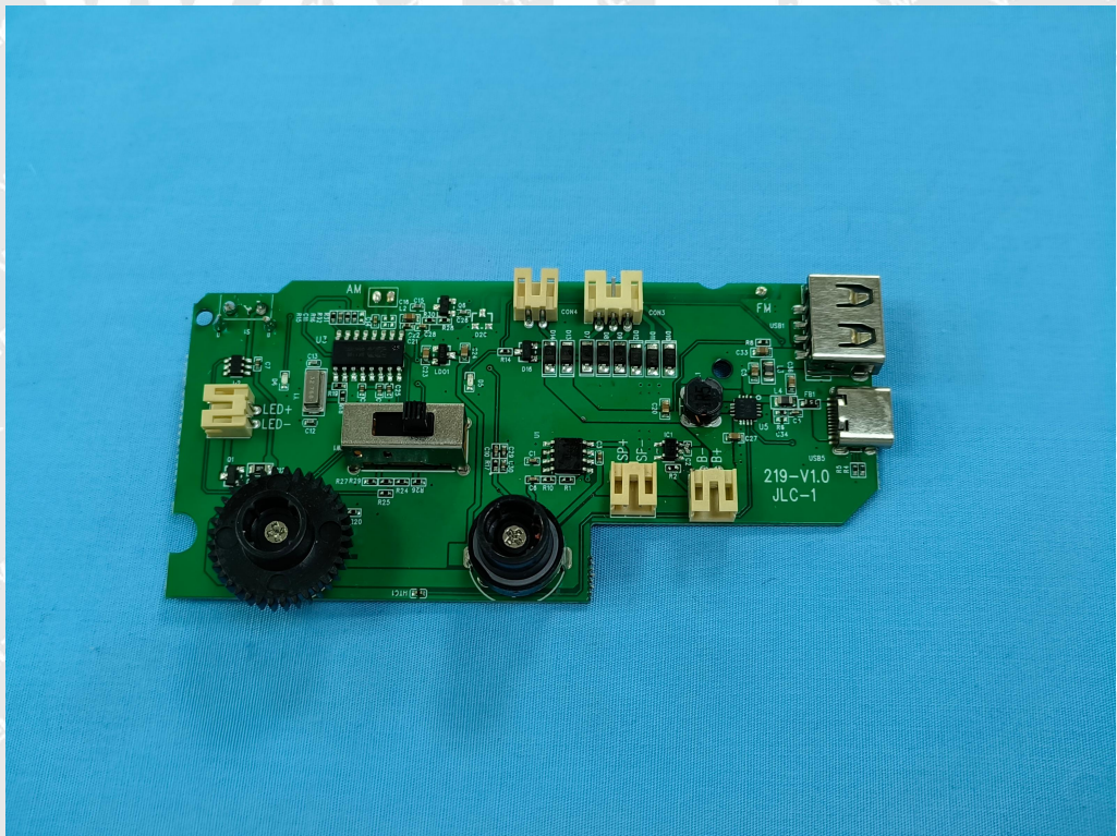
Figure 6 PCB view
