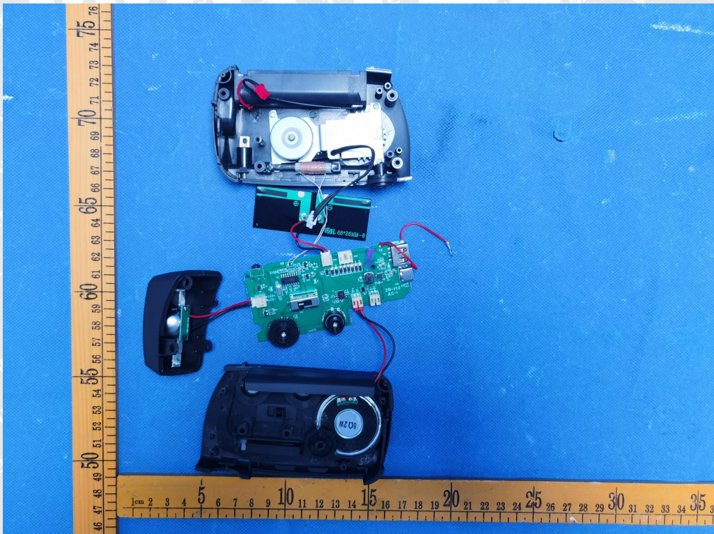
Figure 4 Internal view
