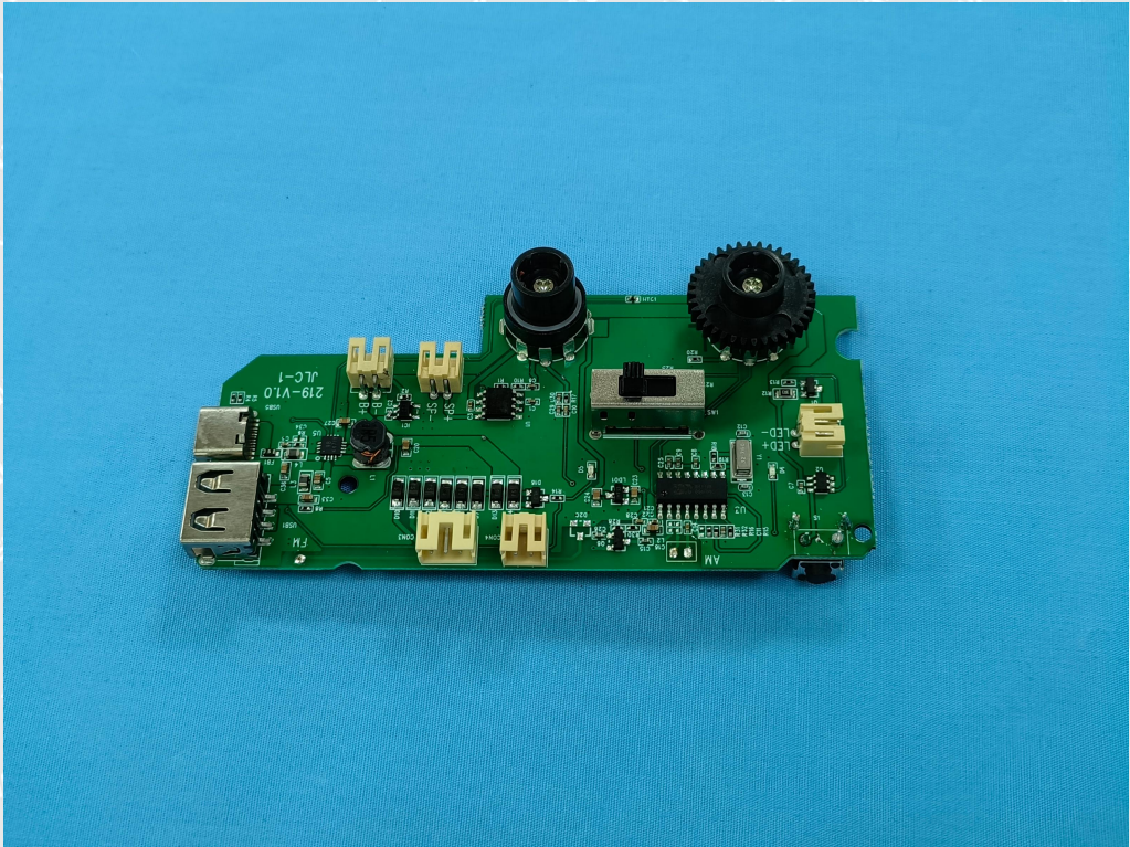
Figure 7 PCB view
