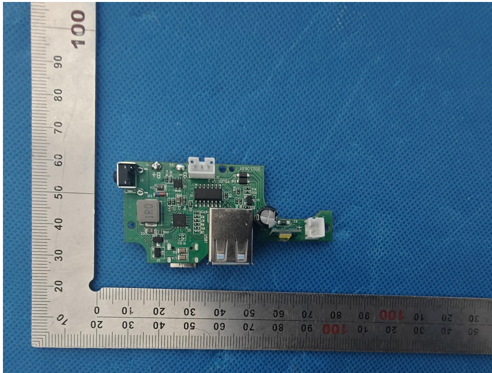
Fig. 7 – PCB view
