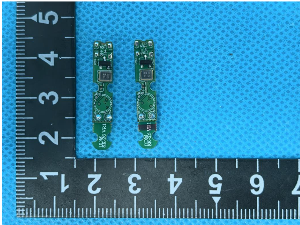
Fig.6 – PCB view (Earbuds)
