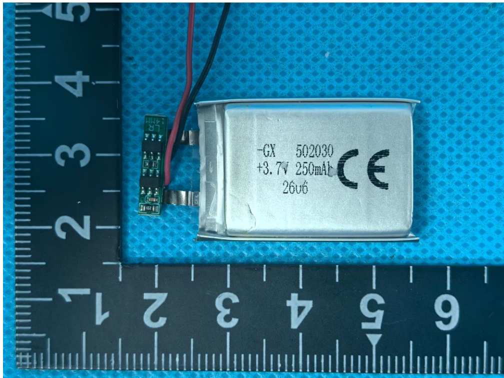
Fig.16 – Battery view (Charge case)
