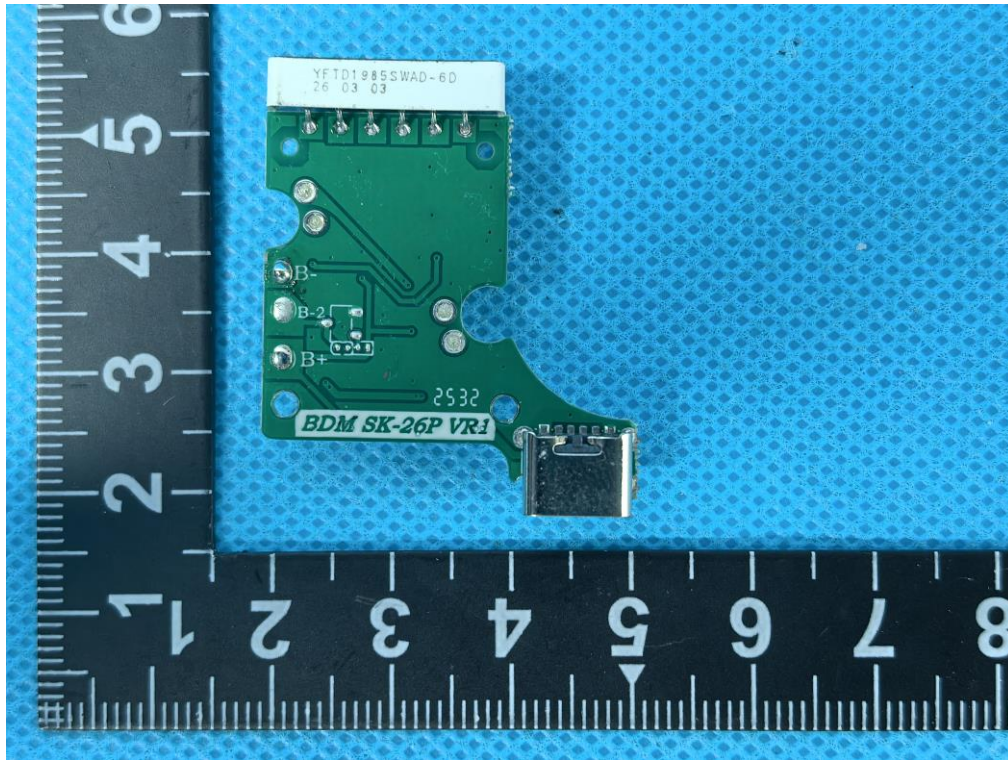
Fig.15 – PCB view (Charge case)
