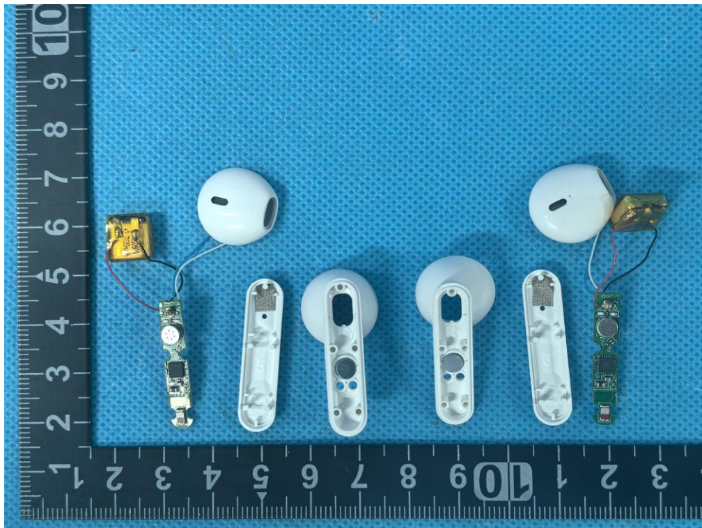
Fig.4 – Open view (Earbuds)
