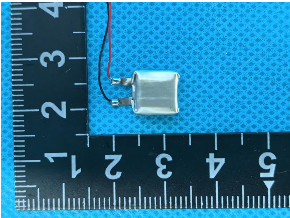
Fig.8 – Battery view (Earbuds)
