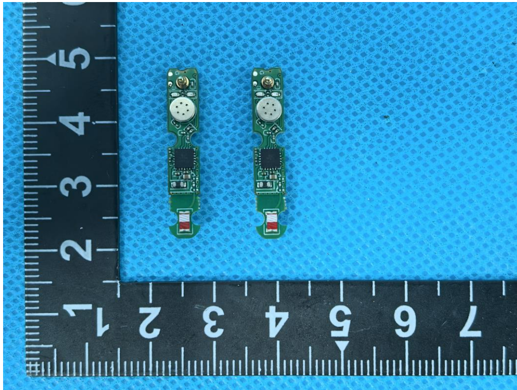
Fig.5 – PCB view (Earbuds)
