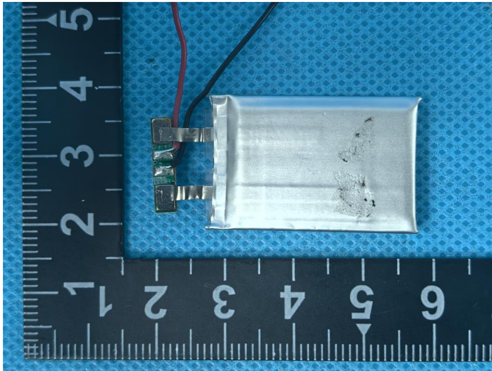
Fig.17 – Battery view (Charge case)
