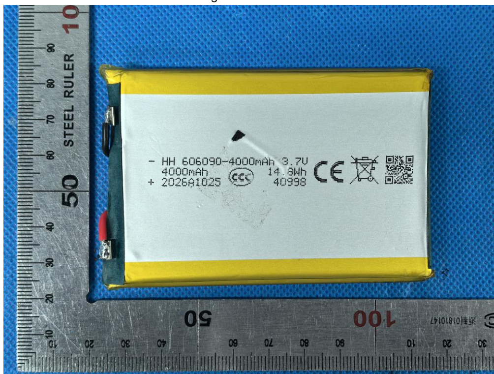
Fig. 8 – Battery view
